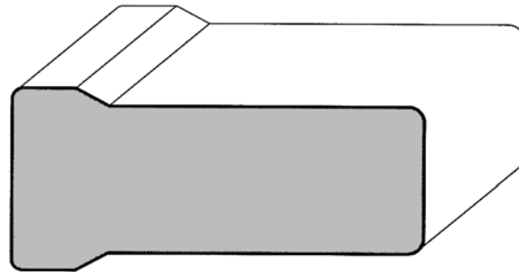
3" Large Bar 1-1/16" x 2-3/8"
